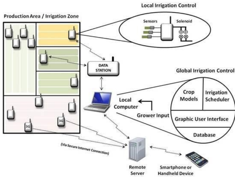
Fig. 1. Graphic of a wireless sensor network, showing radio nodes in production areas, which can be used for local irrigation control, or with environmental sensors for model-based control decisions (From Lea-Cox, 2012).
